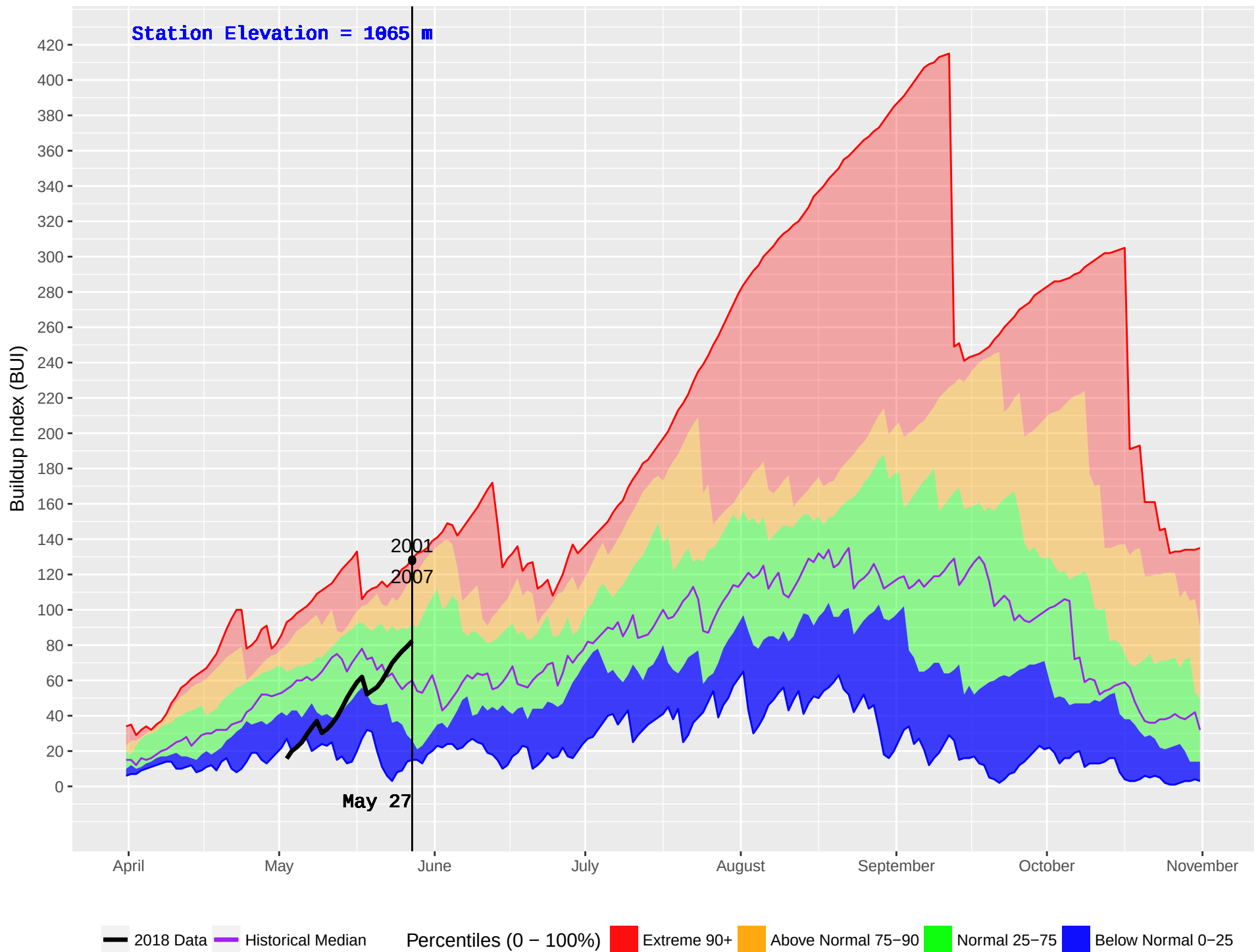
ASPEN GROVE (302) : Historical (1998–2016) and Current (2018) Noon Buildup Index (BUI)
